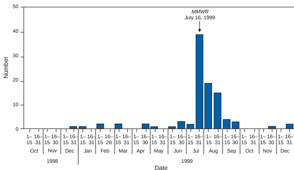
FIGURE 1. Number* of confirmed cases of intussusception after implementation of rhesus-human rotavirus reassortant-tetavalent vaccine, by date reported to the Vaccine Adverse Event Reporting System — United States, October 1, 1998–December 31, 1999
