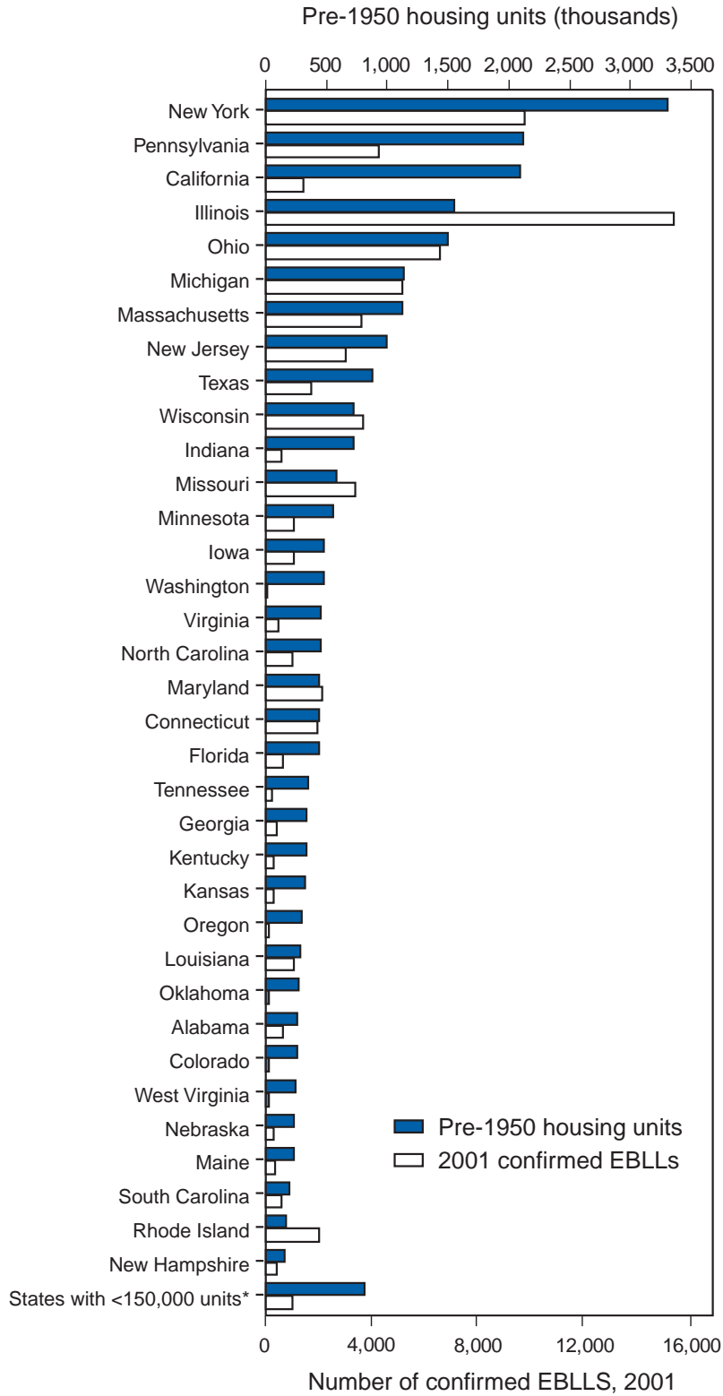
FIGURE 6. Number of pre-1950 housing units and children with confirmed elevated blood lead levels (EBLLs) \geq 10 \mu\text{g/dL} — selected U.S. sites, 2001
