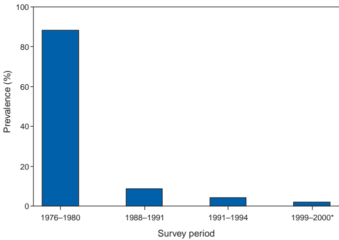
FIGURE 1. Blood lead levels \geq 10 \mu\text{g}/\text{dL} among children aged 1–5 years — United States, 1976–1980, 1988–1991, 1991–1994, and 1999–2000*
