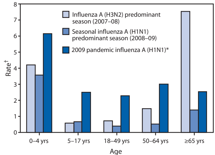
FIGURE 1. Cumulative rate of hospitalizations during three influenza seasons, by age group — Emerging Infections Program, United States, 2007–2010
